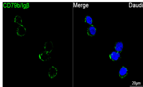
Confocal imaging of Daudi cells using ABflo® 488 Rabbit anti-Human CD79b/Igβ mAb (A23801, dilution 1:200). DAPI was used for nuclear staining (Blue). Objective: 100x.
