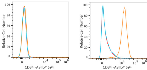
Flow cytometry: 1X10 6 HAP1 cells (negative control,left) and Raji cells (right) were surface-stained with ABflo® 594 Rabbit anti-Human CD84 mAb (A24580,5 µl/Test,orange line) or ABflo® 594 Rabbit IgG isotype control (A23821,5 µl/Test,blue line). Non-fluorescently stained cells were used as blank control (red line).
