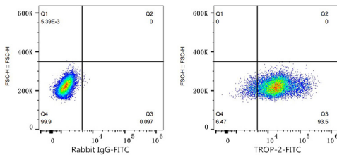
Flow cytometry: 1X10^6 A-431 cells were surface-stained with FITC Rabbit IgG isotype control (5 μl/Test,left) or Goat anti-Human TROP-2 mAb (IgG, κ,right). FITC Rabbit Anti-Goat IgG (Fc) fragment mAb (A25513,5 μl/Test) was used as a secondary antibody.
