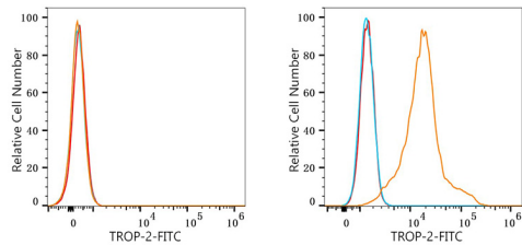
Flow cytometry: 1X10^6 Jurkat cells (negative control,left) and A-431 cells (right) were surface-stained with Goat anti-Human TROP-2 mAb (IgG, κ,orange line) or FITC Rabbit IgG isotype control (5 μl/Test,blue line), followed by FITC Rabbit Anti-Goat IgG (Fc) fragment mAb (A25513,5 μl/Test) staining. Non-fluorescently stained cells were used as blank control (red line).
