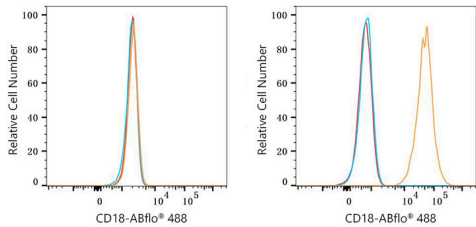
Flow cytometry: 1X10^6 HeLa cells (negative control,left) and THP-1 cells (right) were surface-stained with ABflo® 488 Rabbit anti-Human/Monkey CD18 mAb (A27215,5 µl/Test,orange line) or ABflo® 488 Rabbit IgG isotype control (A22069,5 µl/Test,blue line). Non-fluorescently stained cells were used as blank control (red line).
