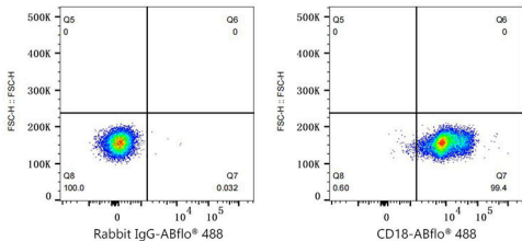
Flow cytometry: 1X10^6 Human PBMC were surface-stained with ABflo® 488 Rabbit IgG isotype control (A22069,5 µl/Test,left) or ABflo® 488 Rabbit anti-Human/Monkey CD18 mAb (A27215,5 µl/Test,right). Cells in the lymphocyte gate were used for analysis.
