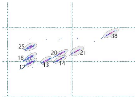
Figure 1. Spectral distribution of capture beads for 8-plex assay.
